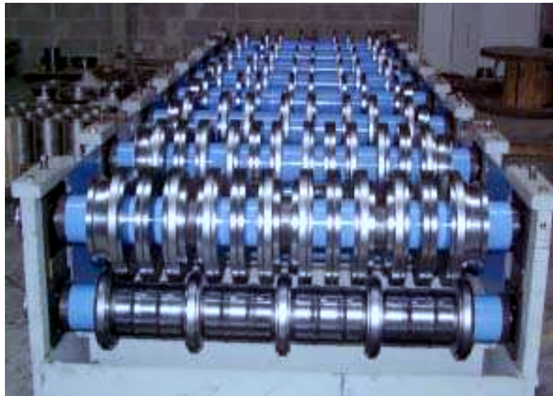
Rollers for sheet shaping Ø180 to 500 mm in tool steel Z200C12 hardened 58/60HRC
