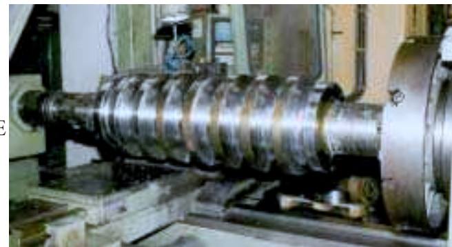
ROLL FOR ROLLER TABLE DURING TURNING PROCESS
